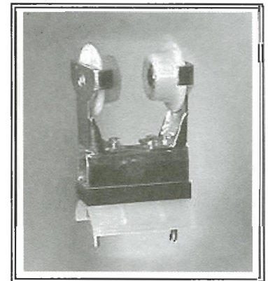
Right: 2-Wheel I-Beam Standard Trolley. Nylon moulded saddle and plated steel trolley to support flat cable. Cables may be stacked in saddle.
