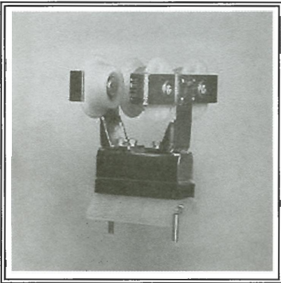
Above: 4-Wheel I-Beam Standard Trolley. Nylon moulded saddle and plated steel trolley to support flat cable. Cables may be stacked in saddle.
